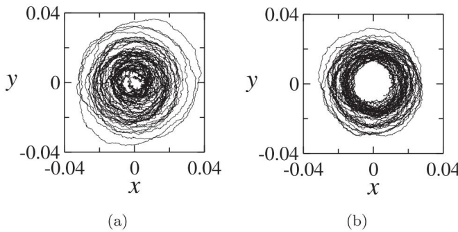
Fig. 1. Numerically simulated phase portraits of noise-induced oscillations of the Van der Pol system at \omega_0 = 1, \varepsilon = -0.01, D = 0.003 : (a) without feedback K = 0 ; (b) with feedback K = 0.2, \tau = T_0 . In both cases the system was integrated during 300 time units.
