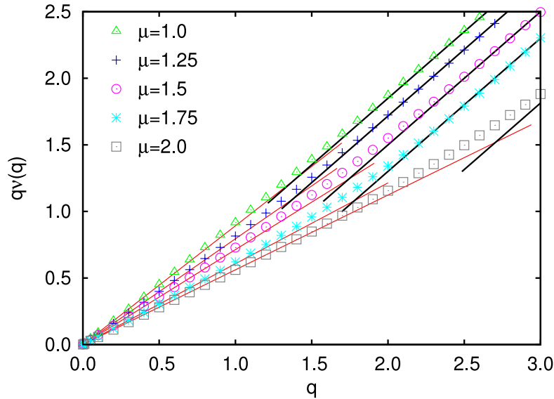
Figure 4. Scaling exponent q\nu(q) for the q th moment of the PDF as a function of q for the velocity model and different exponents \mu . The lines are fits to the behavior of the moments for small or large q , respectively.
