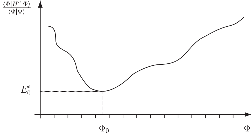
Figure 3.1: Schematic representation of the expectation value of the Hamilton operator as a “function” of the vectors of the Hilbert space of H^e . The tick marks at the \Phi -axis label the wave functions of type \Phi^{\text{Hartree}} . They definitely cannot reach the function \Phi_0 .
