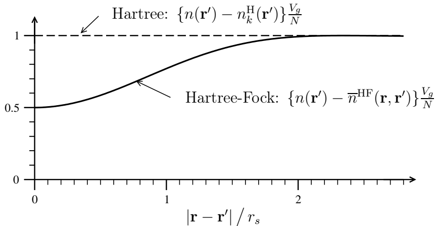
Figure 3.4: Distribution (averaged) of the (N - 1) other electrons with respect to an electron that is located at position \mathbf{r} = 0 (in the Hartree-Fock approximation and for jellium).
