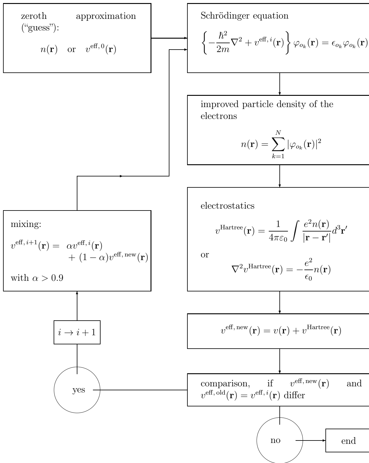
Figure 3.2: Scheme of the self-consistent field method for the solution of the Hartree equation. Here, v^{\text{SIC}} has been neglected. Analogous diagrams exist for Hartree-Fock and density-functional theory.
