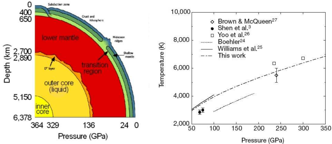
Figure 3.18: A cut through the earth showing the various shells (left) and the calculated melting curve for iron. (D. Alfè, G.D. Price, and M.J. Gillan, “Melting curve of Iron at Earth’s core pressures from ab-initio calculations”, Nature 401 , 462-464 (1999).)
