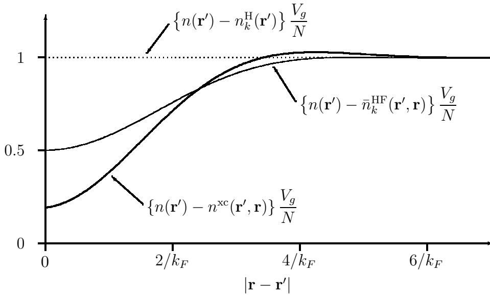
Figure 3.15: The exchange-correlation hole for jellium. n^{\text{xc}}(\mathbf{r}', \mathbf{r}) is shown schematically.
